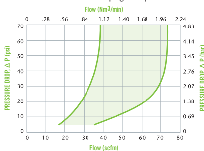
APC AIR FLOW • 100 psig inlet pressure
