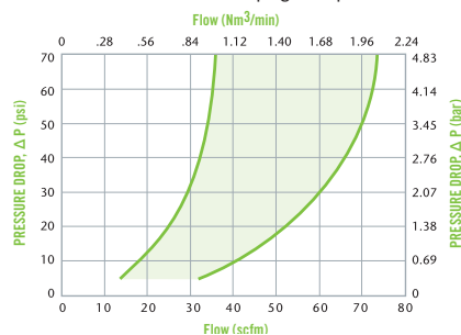
EFC12 AIR FLOW • 100 psig inlet pressure
