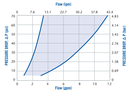
PLC WATER FLOW
